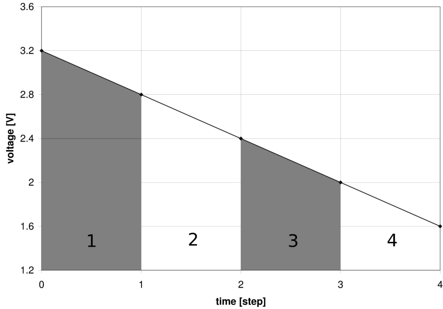
Figure 1: The voltage drop for a battery pack consisting of two AA cells while discharging with a constant current. The areas 1, 2, 3 and 4 represent the percentage of the energy available in each voltage range
